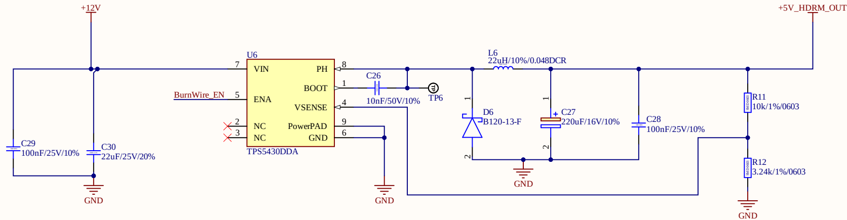
BurnWire Power Regulation
