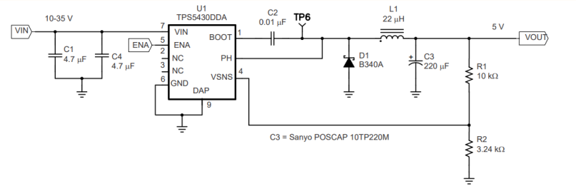
Figure 7-9. 10-V – 35-V Input to 5-V Output Application Circuit
