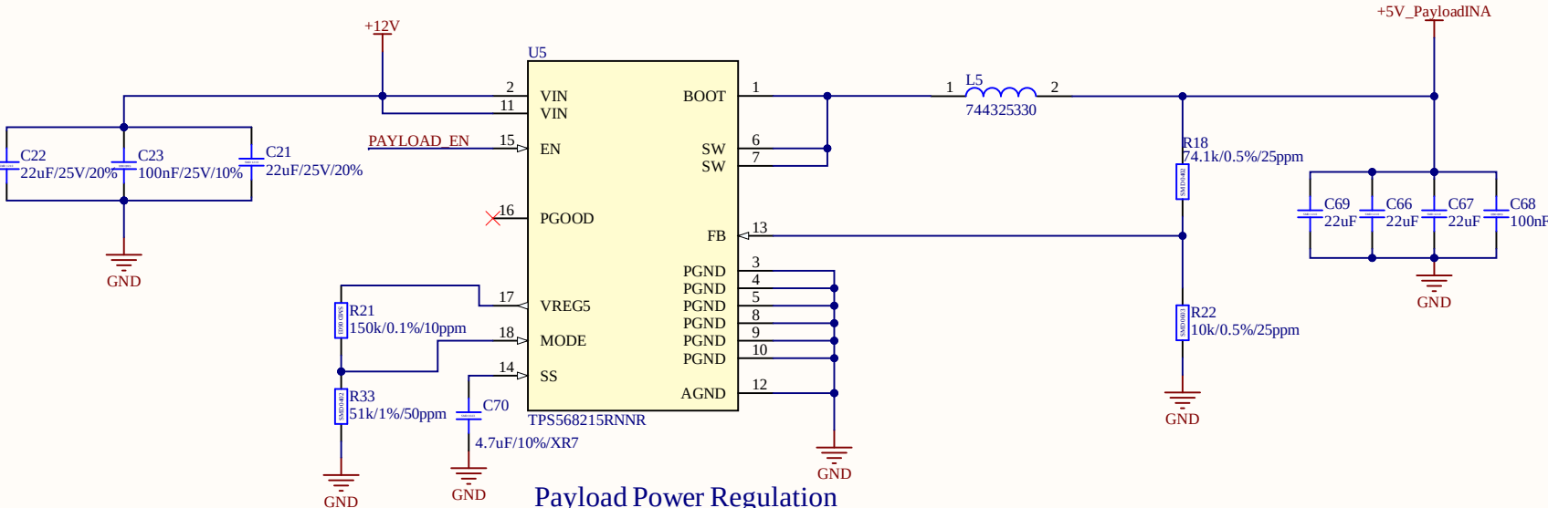
Payload Power Regulation
