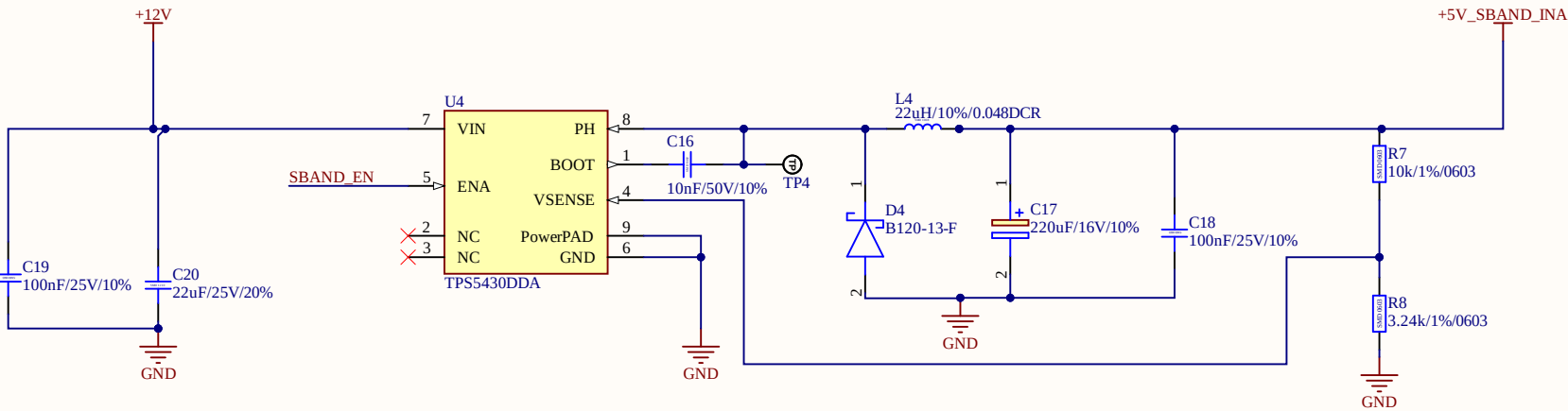
SBAND Power Regulation
